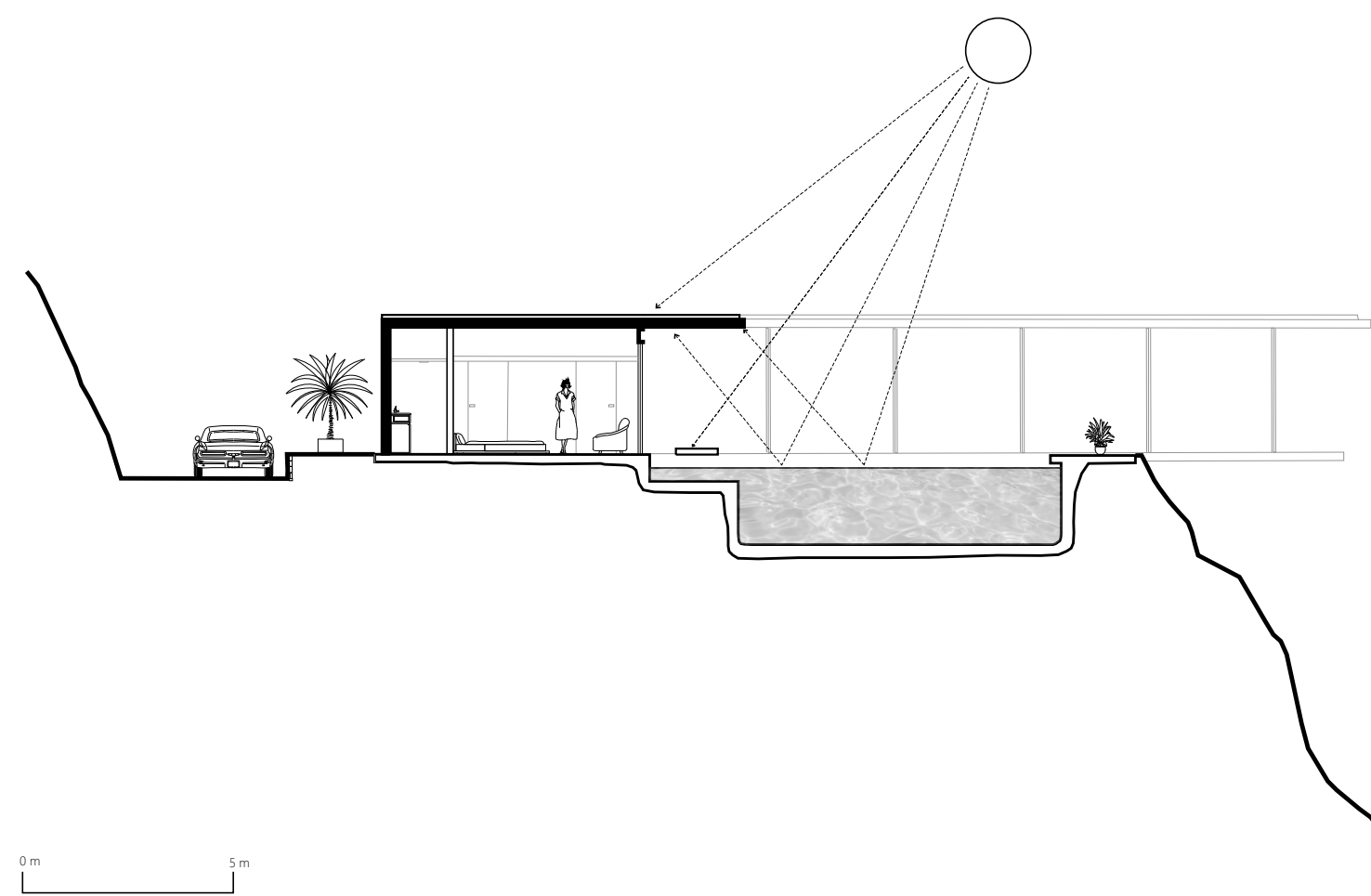
Pool Light Reflection Section B - B'
